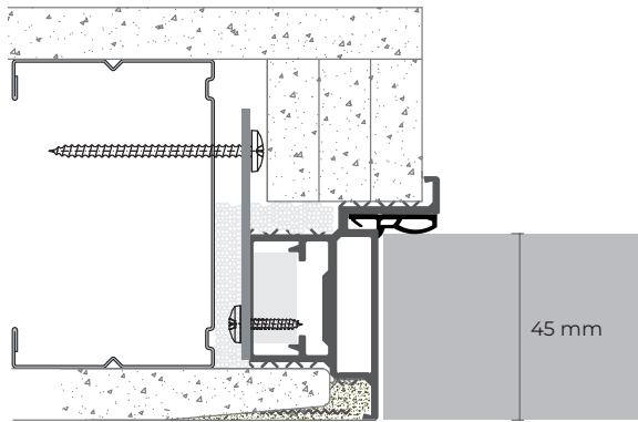
45 mm - a tirare 45 mm - pull version
