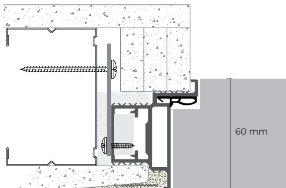
60 mm - a tirare 60 mm - pull version
